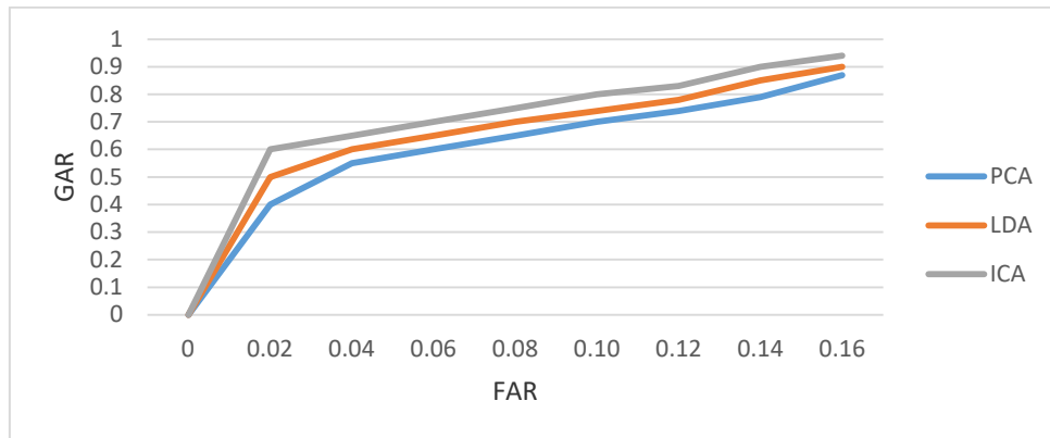
Fig. 2: ROC Curve for GAR and FAR
