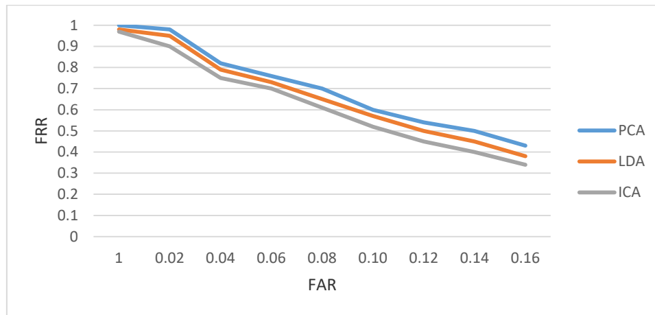
Fig. 3: ROC Curve for FAR and FRR
