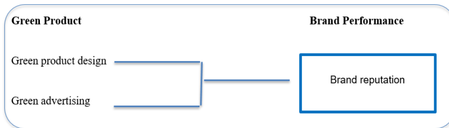
Fig 1: Conceptual framework
