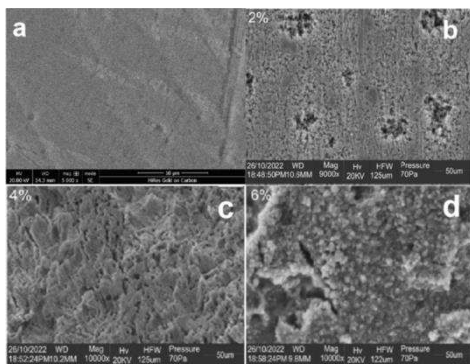
Fig. 6 Scanning electron micrograph of: (a) base aluminum alloy (b) + 2wt% of Okaba coal ash (c) + 4wt% of Okaba coal ash (d) +6wt% of Okaba coal ash
