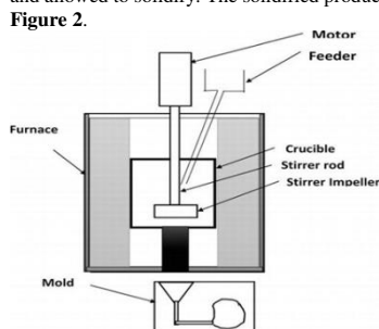
Fig. 1 Stir casting set-up
