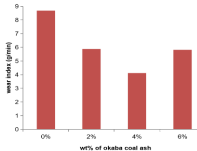
Fig. 4 Effect of OCA wt.% on the wear index for 500 g at 1000 rpm
