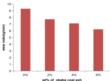
Fig. 5 Effect of OCA wt.% on the wear index for 750 g at 1000 rpm
